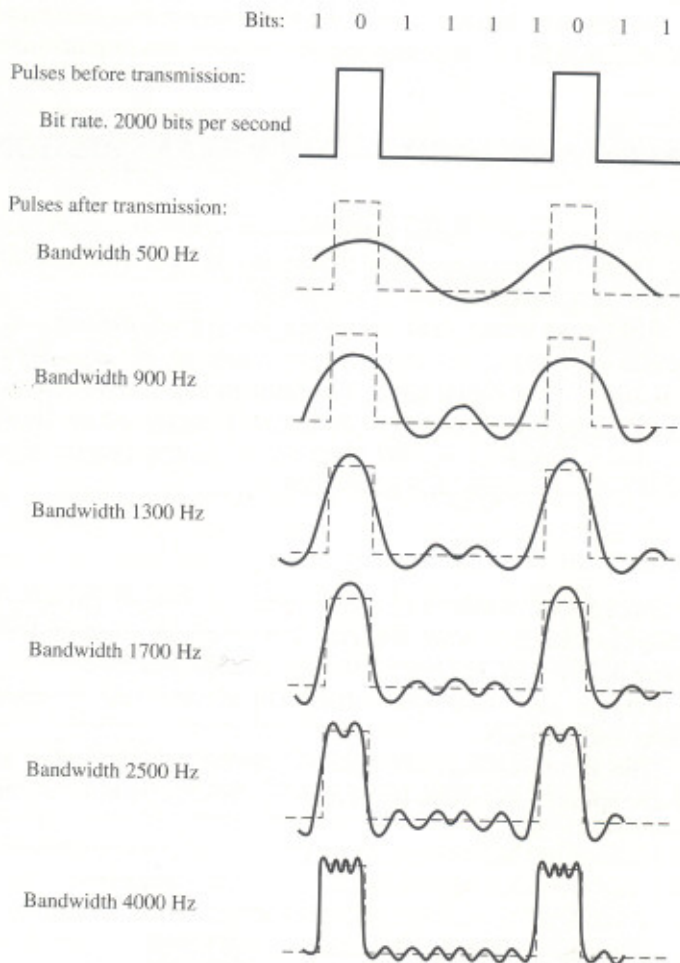
Figure 3.8 Effect of Bandwidth on a Digital Signal
